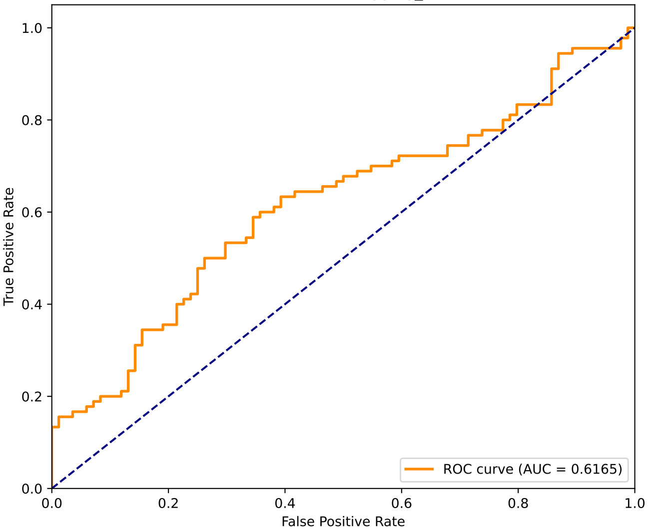
ROC Curve - Bagging_LR
